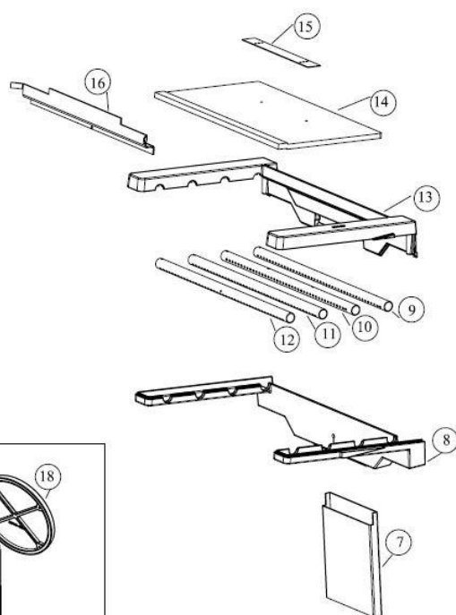
ASSEMBLY B: SECONDARY AIR
