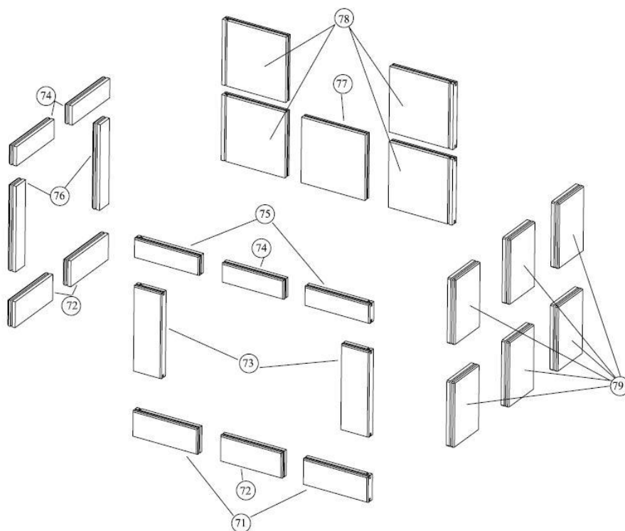
ASSEMBLY D: VERTICAL STONE
